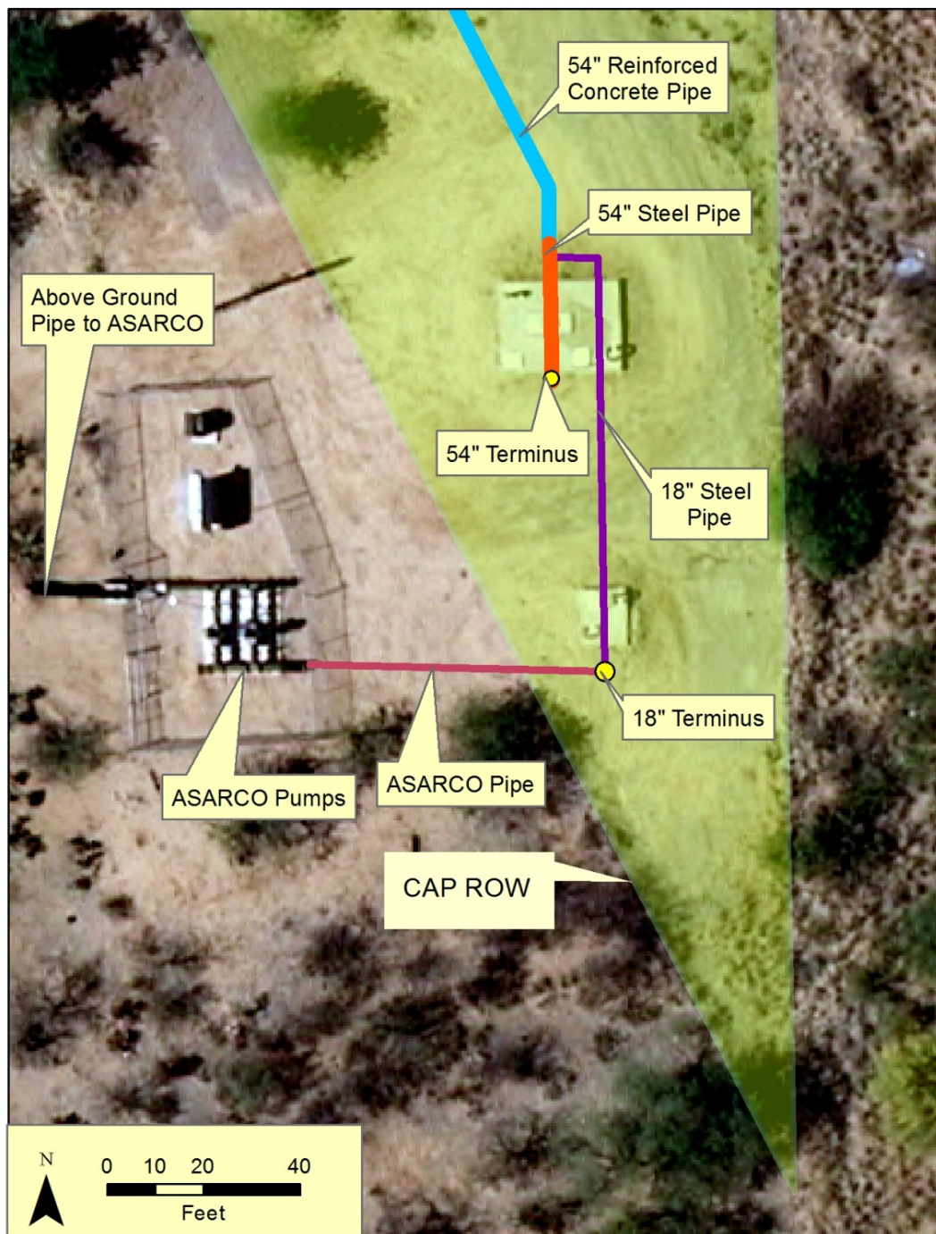
Figure I-7 – Plan View of CAP Terminus
