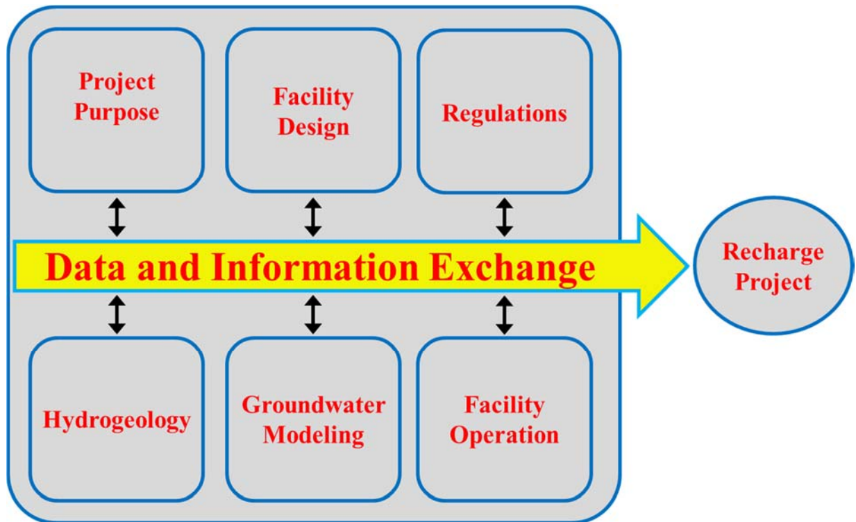
Figure 7 - Conceptual Diagram of the Process to Locate and Permit a Recharge Facility in Arizona
