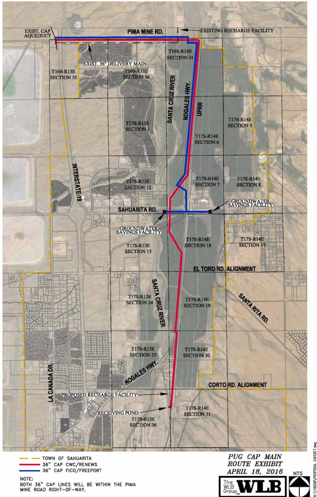
Figure 4 - Proposed CAP Pipelines
