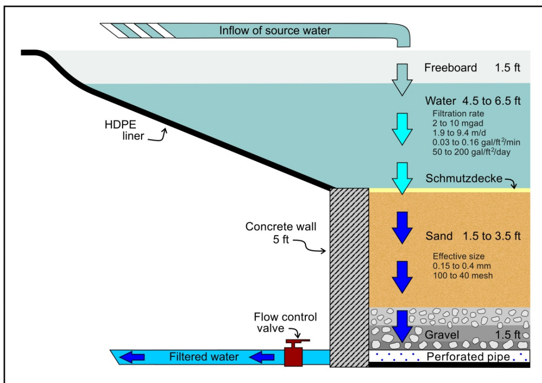
Figure 5 - Diagram of a Typical Slow-Sand Filtration System
