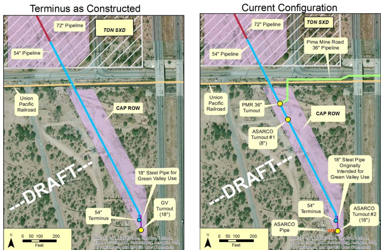
Figure I-6 - CAP Terminus as Constructed and Current Configuration
