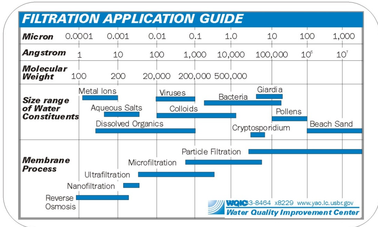
Figure 6 - Typical Water Constituents and Processes for Removal
